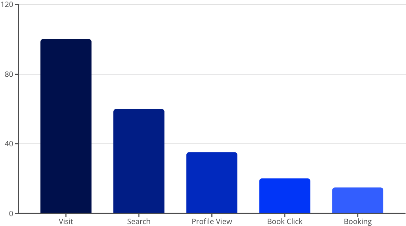
Funnel Metrics
